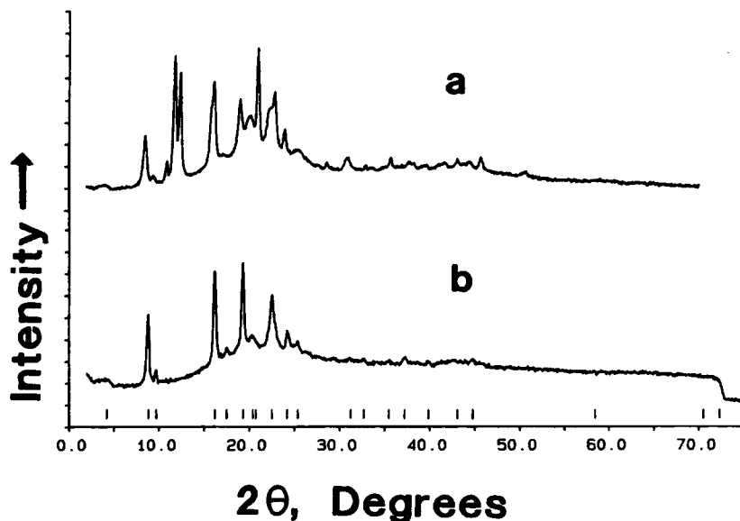
Fig. 8. Wide angle X-ray powder diffraction scan of polyBEMO: (a) as received; (b) crystallized from the melt, T_1 = 100^\circ\text{C} , at 35 and 60^\circ\text{C} .
