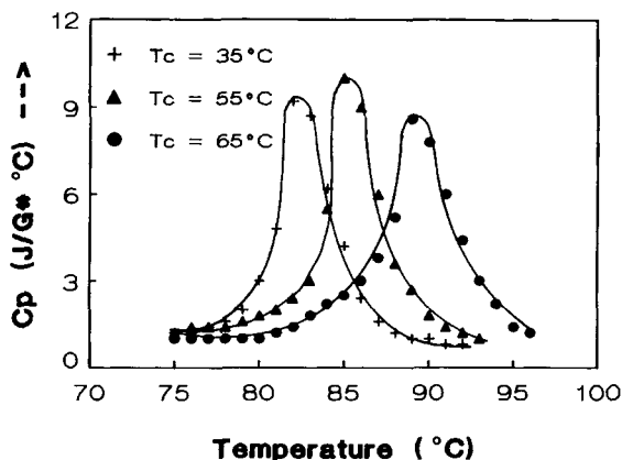
Fig. 1. DSC thermogram of polyBEMO crystallized at different temperatures. T_l = 100^\circ\text{C} .
