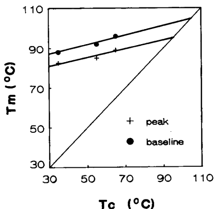
Fig. 2. Hoffman-Weeks plots for polyBEMO.
