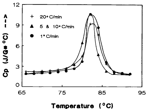
Fig. 3. Effect of DSC heating rate on polyBEMO.
