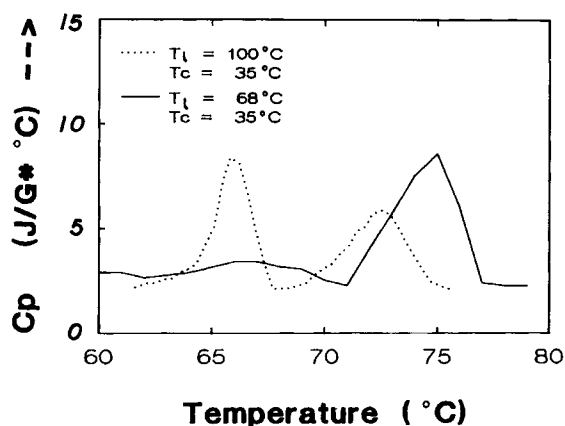
Fig. 6. DSC thermogram showing the effect of partial melting and recrystallization on the melting behavior of polyBEMO sample #2.
