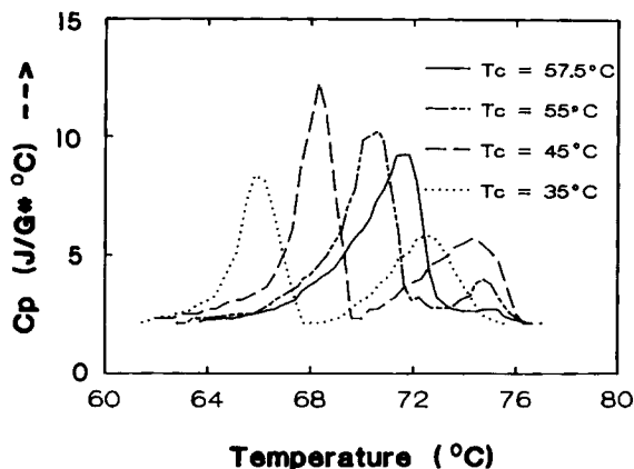
Fig. 4. Effect of crystallization temperature on the melting behavior of polyBEMO sample #2. T_1 = 100^\circ\text{C} .
