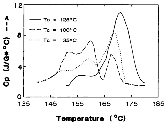
Fig. 9. DSC thermogram showing the effect of crystallization temperature on the melting behavior of polyBCMO. T_1 = 220^\circ\text{C} .
