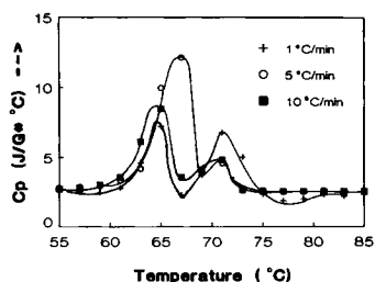
Fig. 5. Effect of heating rate on polyBEMO sample #2. T_c = 35^\circ\text{C} ; T_i = 100^\circ\text{C} .
