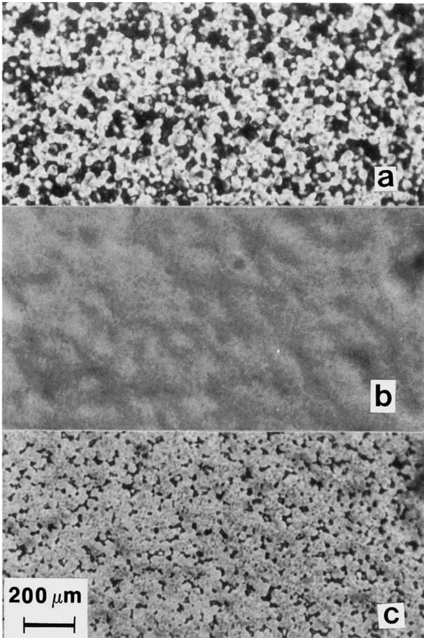
Fig. 7. Optical microscopy of polyBEMO sample #3.
